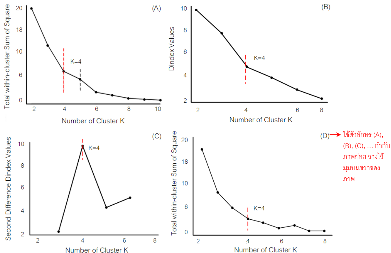
Figure 3 Determination the best number of clusters; (A) WSS value, (B) Index in NbClust, (C) Second Different Dindex NdClust, (D) Elbow Method
